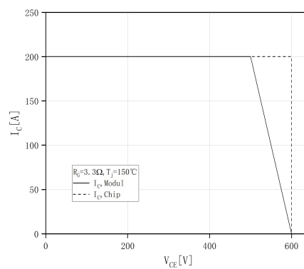
反偏安全工作区 IGBT, 逆变器 (RBSOA) Reverse bias safe operating area IGBT, Inverter(RBSOA)
