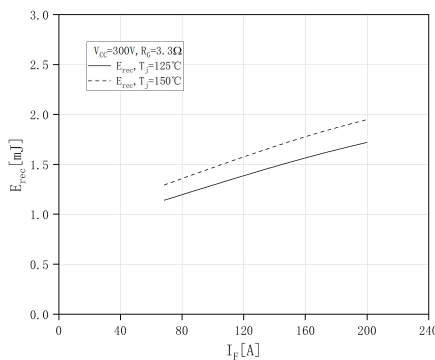
开关损耗 二极管,D5-D6 (典型) switching losses Diode, D5-D6(typical)
